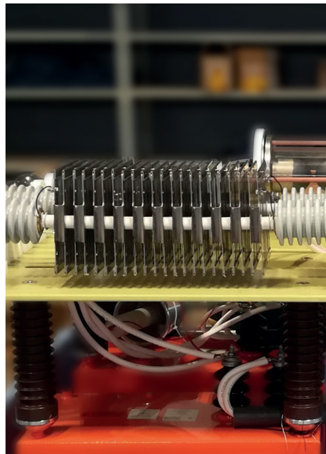
150 kJ Bank
